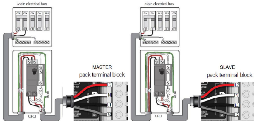
240 V (4 wires) Refer to wiring diagram in the enclosure box lid for more information.
